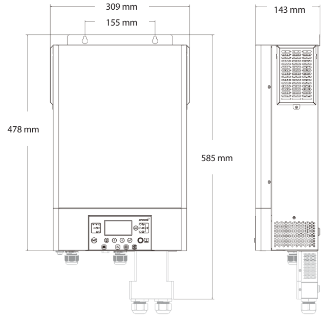
230 Vac models and PSW-H-3KW-120/24V*
