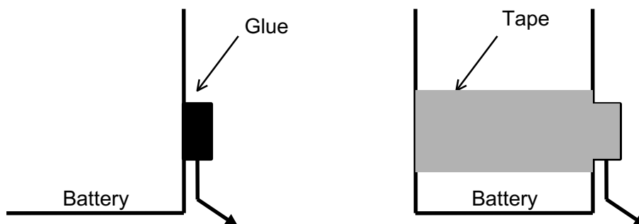
Figure 0-2 - Sensor Installation
